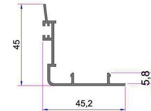
Alm. Super Sash Cover Profile AD16-032
