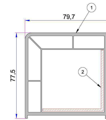
Universal Short Coupling Profile P.A.099.5004.600
