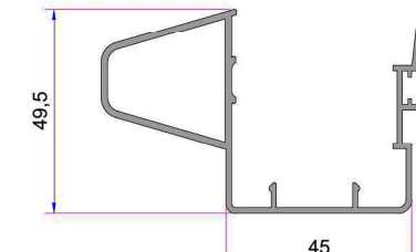
Alm. Sash Cover Grillage Profile (In Process)
