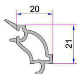
4mm Single Glazing Bead P.A.101.4102.600.0.00.01
