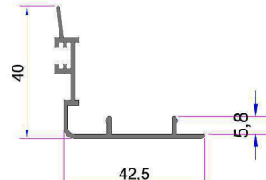
Alm. Sash Cover Profile AD16-031
