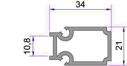
Alm. Double Rail Adaptor AD16-011
