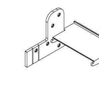
Aluminium Frame Threshold Wedge 221013.0000.L - 221013.0000.R
