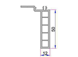
50mm Frame Sill Profile P.A.099.5524.600.0.00.19
