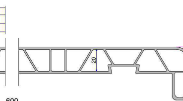
PVC Sill Profile (600mm) P.DNZ.01.60.E.600.19
