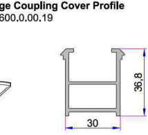
Frame Montage Profile P.A.060.5301.600.0.00.19
