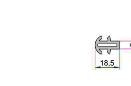
Short Coupling Profile P.A.099.5003.600.0.00.19
