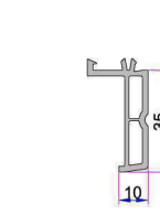
35mm Frame Sill Profile P.A.099.5523.600.0.00.19
