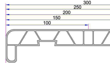
PVC Sill Profile (600mm) P.DNZ.01.60.E.600.19
