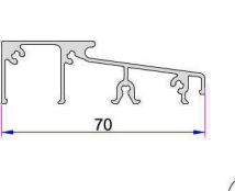
Frame Seal
