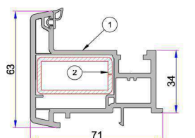
Lap Joint Cover Profile 34012-10140
