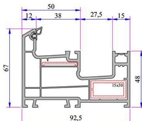
Frame Profile (Single Rail) P.A.232.1105.600.0.BC.03
