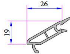
Single Glazing Bead (4mm) P.A.332.4000.600.0.HC
