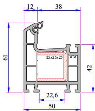
332 Frame Profile P.A.332.1000.600.0.BC.03
