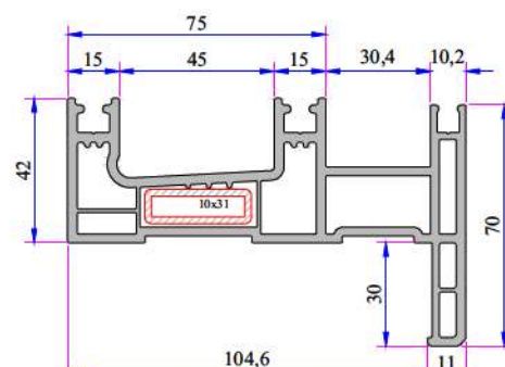
Frame Profile With Internal Fly-Screen P.A.242.1104.600.0.00.03
