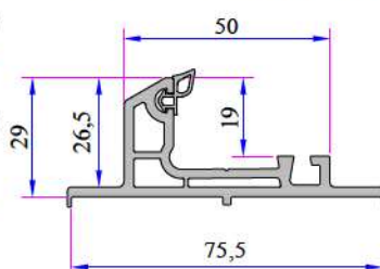
Double Rail Adaptor Profile P.A.232.5800.600.0.BC.19
