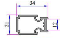
Alm. Double Rail Adaptor Profile AD16-011 (White)
