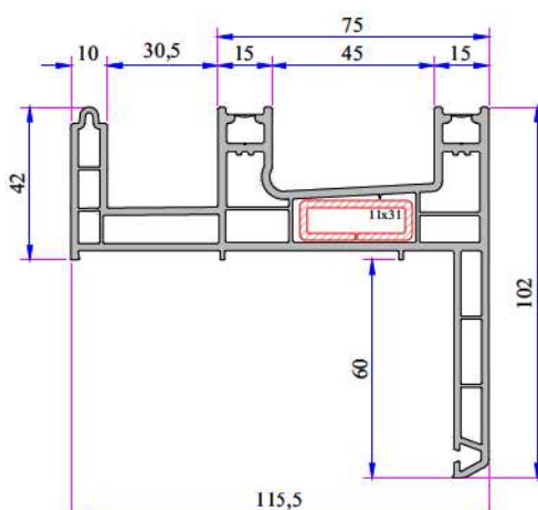
Double Rail Frame Profile With Fly - Screen 60 mm Sill P.A.232.1115.600.0.BC.03
