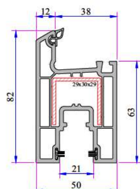
Sliding System Sash Profile P.A.232.2300.600.0.BC.03
