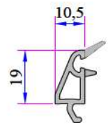
Double Glazing Bead (20mm) P.A.332.4100.600.0.HC
