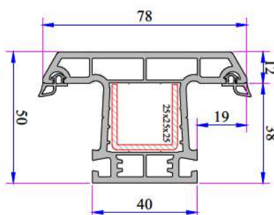
332 Mullion Profile P.A.332.3000.600.0.BC.03
