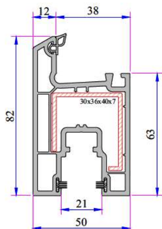
Sliding System Sash Profile (Static) P.A.232.2308.111.0.BC.01
