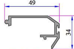
Alm. Cover Profile 16013.601.5.2.0.0000
