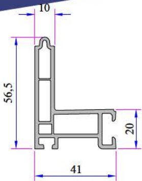
Screen Adaptor Profile P.A.232.5802.600.0.00.19
