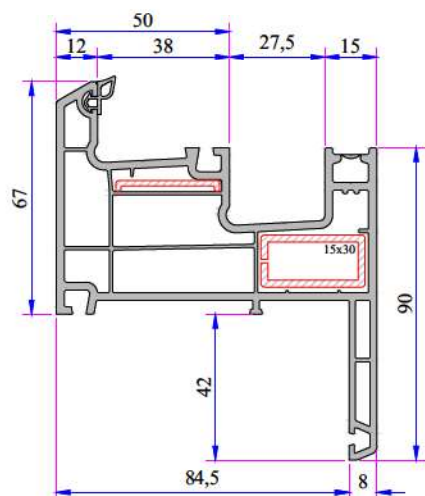
Frame Profile With Sill (Single Rail) P.A.232.1114.600.0.00.03
