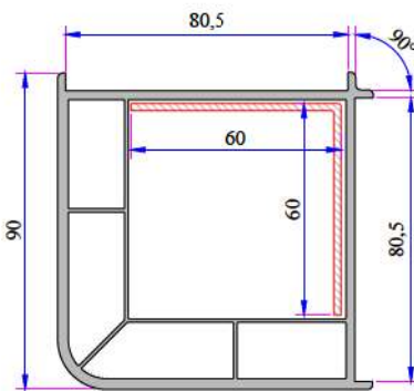
90° Corner Profile (White) P.A.080.5100.600.0.00.19
