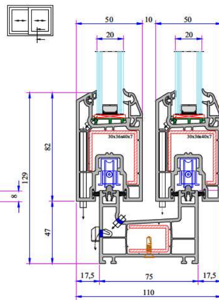
Sliding Frame Static Sash Double Rail Installation
