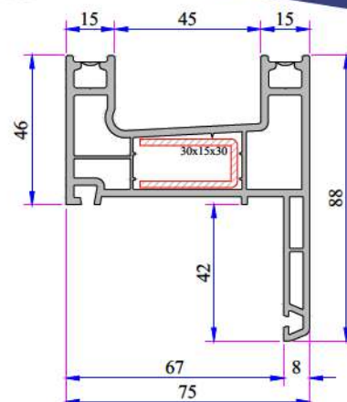
Frame Profile With Flat Sill P.A.232.1110.600.0.00.03
