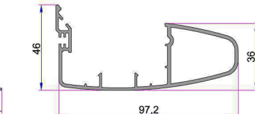
Alm. Sash Cover Grillage Profile 16028.601.5.2.0.9016
