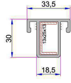
Fly-Screen Mullion Profile P.A.242.3200.600.0.00.01
