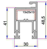
Fly-Screen Sash Profile P.A.242.2305.600.0.00.01
