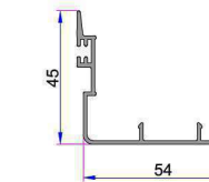
Alm. Sash Cover Profile 16051.601.5.1.1.9016
