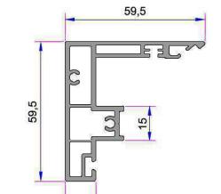
Alm. Sliding Mullion with Three Chambered (In Process)
