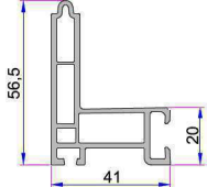
Screen Adaptor Profile P.A.232.5802.600.0.00.19
