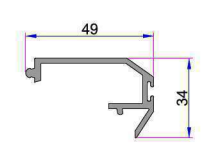
Alm. Cover Profile AD 16 - 013
