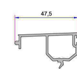
Single Rail Cover Profile P.A.232.5710.600.0.00.19
