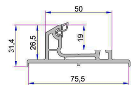
Double Rail Adaptor Profile P.A.232.5800.600.0.BC.19
